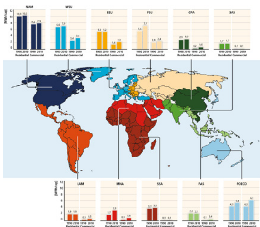
FIGURE 1. Annual per capita final energy use of residential and commercial buildings for eleven regions (GEA RC11, see Annex II.2.4) in 1990 and 2010. Data from (IEA, 2013). Lucon and Urge-Vorsatz et al, Mitigation in Buildings, in “Climate Change 2014: Mitigation of Climate Change,” Intergovernmental Panel on Climate Change Working Group III (2014); Available at: http://report.mitigation2014.org/drafts/final-draft-postplenary/ipcc_wg3_ar5_final-draft-postplenary_chapter9.pdf
